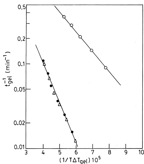
Figure 9 Log t_{gel}^{-1} versus 1/\Delta T_{gel} plots of PVF 2 gels (4 g/dL) in GTB: ○—KY-201, ●—Sol-12 and △—Sol-10
